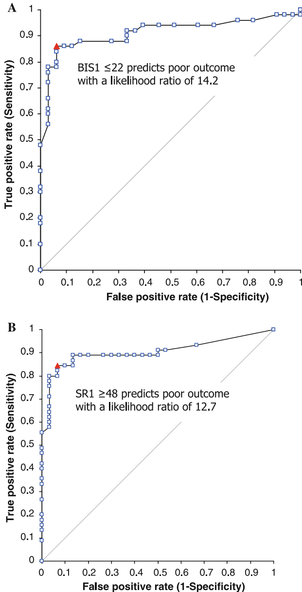
Fig. 2 a Receiver-operator characteristic (ROC) curve describing the accuracy of BIS1 to predict poor neurological outcome. The area under the curve (AUC) is 0.91 (95% CI 0.85–0.98, p < 0.001 ). At a cutoff point of \text{BIS1} \leq 22 (red triangle), the likelihood ratio (LR) of a poor outcome was 14.2 (sensitivity 0.86 and specificity 0.94). b ROC curve describing the accuracy of SR1 to predict a poor neurological outcome. The AUC is 0.90 (95% CI 0.83–0.98, p < 0.001 ). At a cutoff point of \text{SR1} \geq 48 (red triangle), the LR of a good outcome was 12.7 (sensitivity 0.84 and specificity 0.93)
